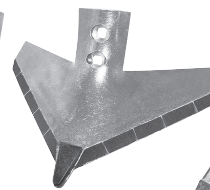
Soc triangle type Boisselet
